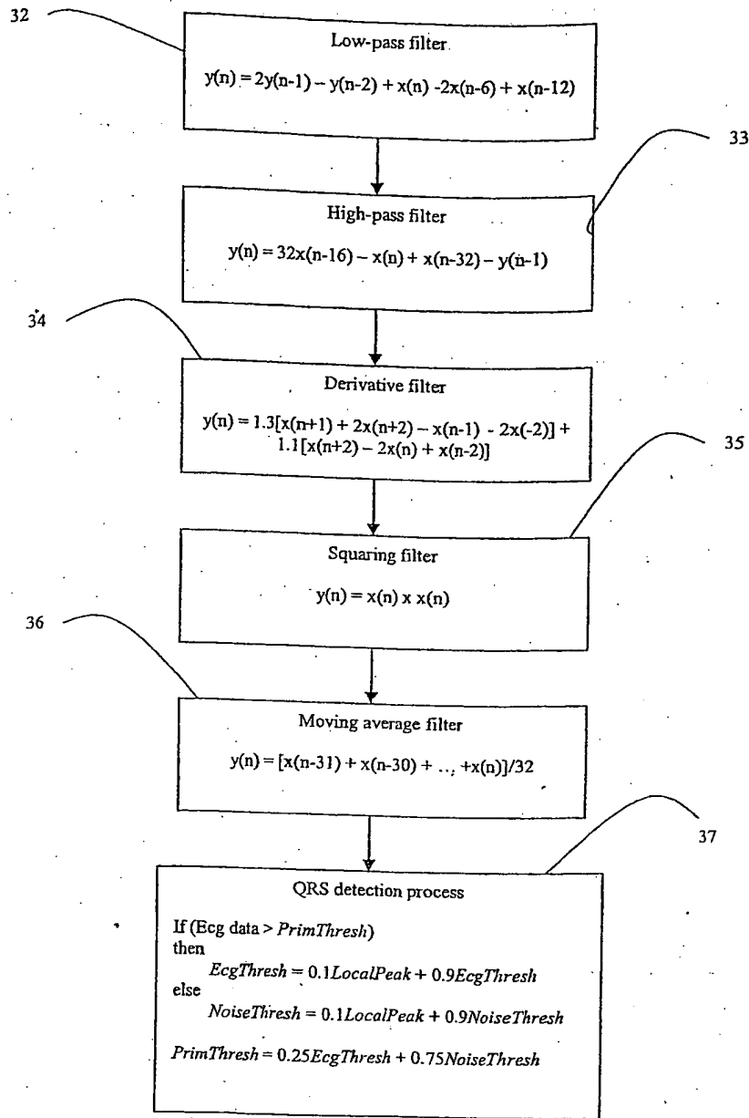
Figure 6b: ECG digital filtering process
